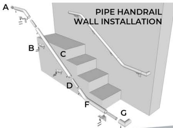
G. 90° Pipe Handrail Return Kit
